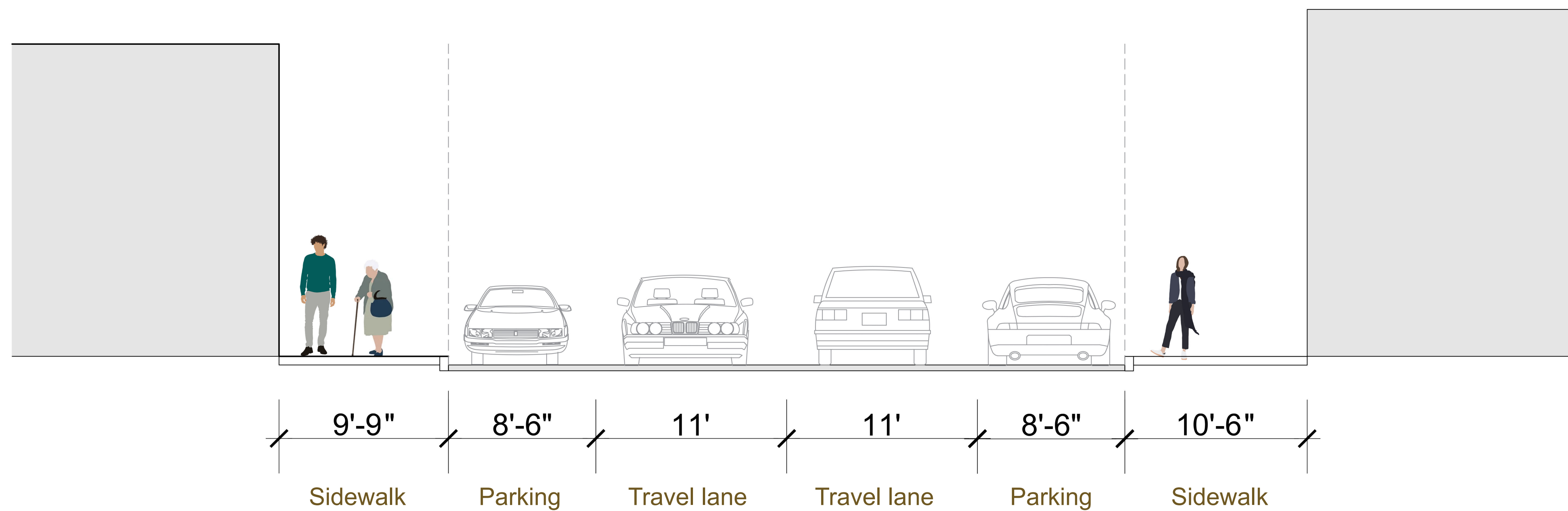
POSSIBLE SECTION
