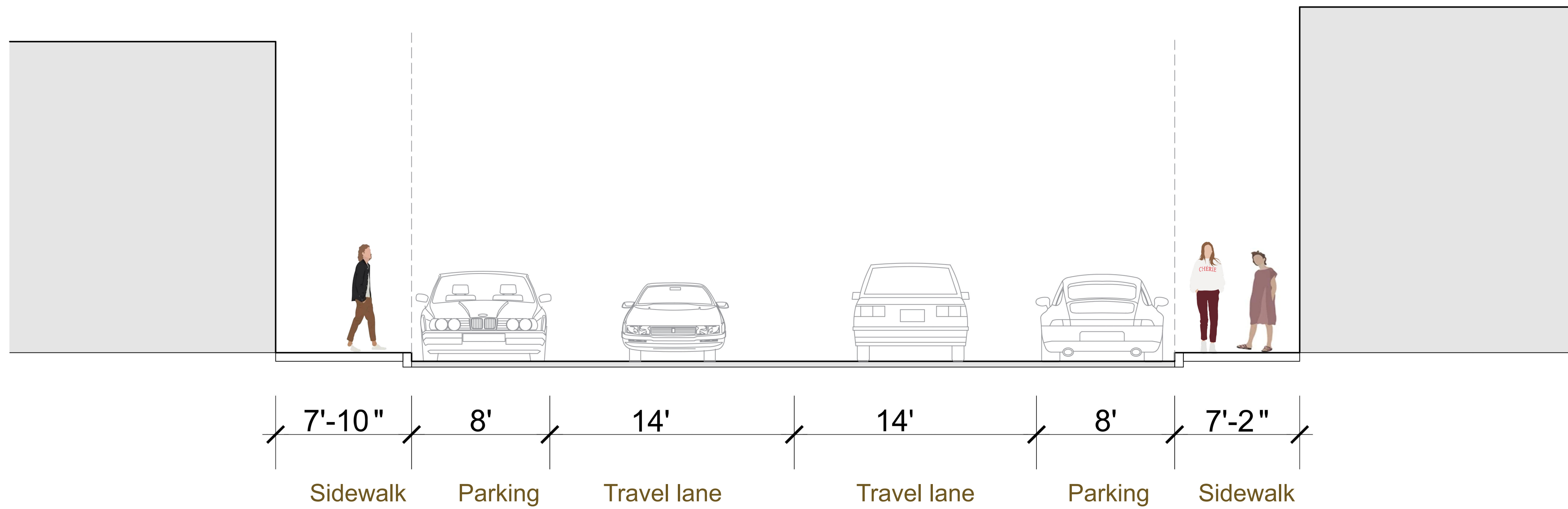
EXISTING SECTION
