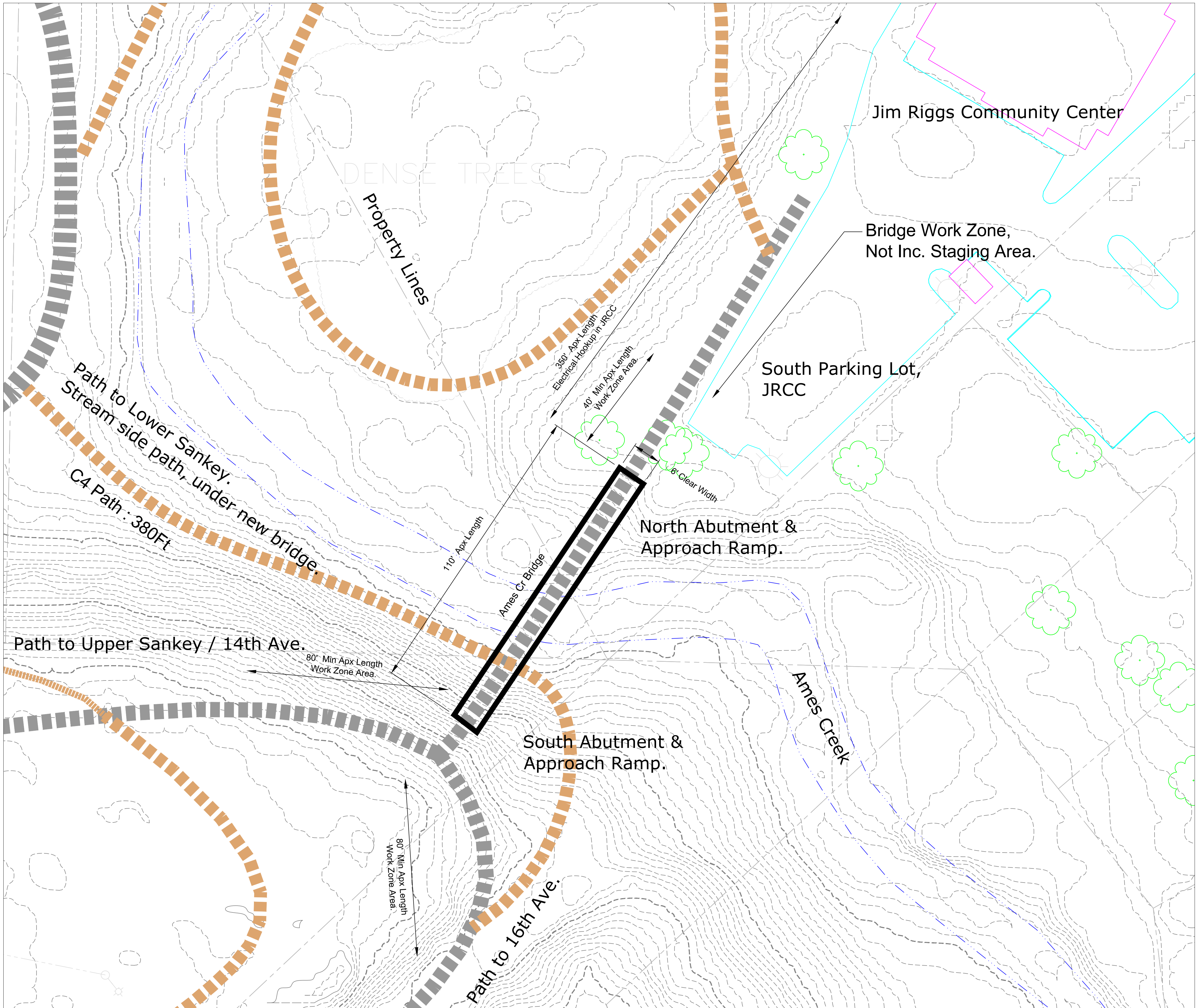
Project Overview - Ames Creek Bridge Horizontal Scale 1" = 50'
